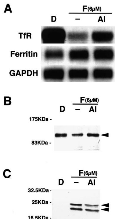
Fig. 2. Aluminum stimulates Tfr production by stabilizing its mRNA and suppresses ferritin biosynthesis in MEL cells. A: MEL cells were treated with 6 μM FAC (F) in the presence (Al) or absence (–) of 100 μM AlCl 3 for 48 h. Control cells were treated with 100 μM Df for 16 h (D). Northern blot for Tfr, ferritin H chain, and GAPDH RNA levels in MEL cells were performed. B, C: MEL cells were treated under the same condition as in A. Cells were labelled metabolically, and biosynthesis of Tfr or ferritin was assessed as described in Section 2. Arrows indicate Tfr (B) or ferritin H and L chains (C).
