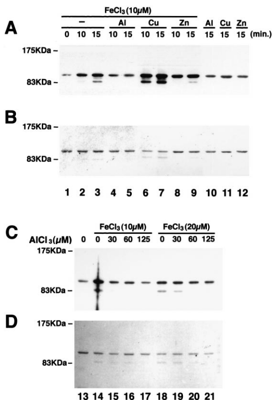
Fig. 4. Aluminum chloride inhibits the iron-induced oxidation of IRP2 in vitro. A: 4 \mu g of recombinant IRP2 was incubated with 10 \mu M FeCl 3 and 10 mM DTT for 10 or 15 min in the absence (lanes 2, 3) or presence of 125 \mu M AlCl 3 (lanes 4, 5), 125 \mu M CuSO 4 (lanes 6, 7), or 125 \mu M ZnSO 4 (lanes 8, 9) together with 10 mM DTT at 37°C. Or, IRP2 was incubated with 125 \mu M AlCl 3 (lane 10), 125 \mu M CuSO 4 (lane 11), or 125 \mu M ZnSO 4 (lane 12) in the presence of 10 mM DTT for 15 min at 37°C. Oxidative modifications of IRP2 were assessed by the assay for carbonyl detection together with non-treated IRP2 (lane 1) as described in Section 2. B: The same membrane was stained with Coomassie brilliant blue. C: 4 \mu g of recombinant IRP2 was incubated with the indicated concentrations of AlCl 3 and 10 mM DTT in the presence of either 10 \mu M (lanes 14–17) or 20 \mu M (lanes 18–21) FeCl 3 for 15 min at 37°C. Oxidative modifications of IRP2 were monitored and compared with non-treated IRP2 (lane 13). D: The same membrane was stained with Coomassie brilliant blue.
