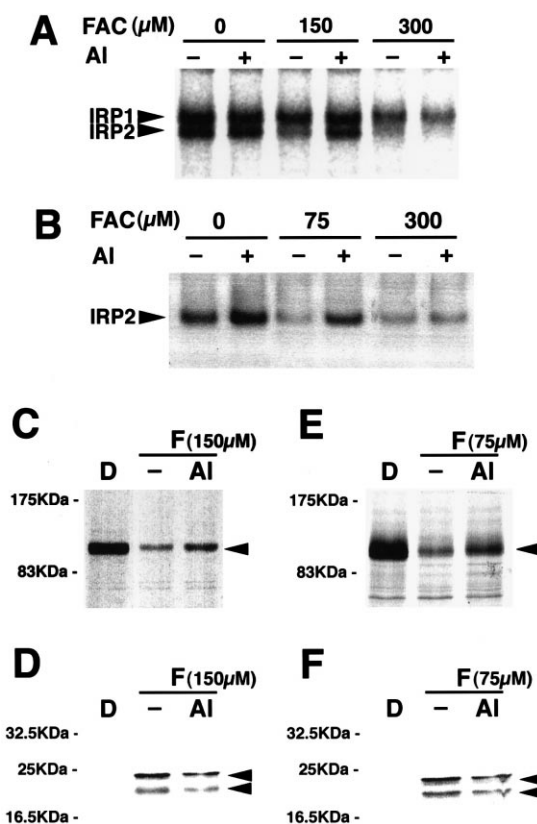
Fig. 3. Aluminum suppresses ferritin biosynthesis and increases Tfr production via increased IRE binding activity of IRP2 in Neuro 2A cells and Ba/F3 cells. Neuro 2A cells (A) or Ba/F3 cells (B) were incubated with the indicated concentration of FAC in the presence (+) or absence (–) of 500 μM of AlCl 3 for 48 h. Lysates were assessed by gel retardation assays (A, B). Neuro 2A cells (C, D) or Ba/F3 cells (E, F) were incubated with (Al) or without (–) 500 μM AlCl 3 in the presence of 150 μM or 75 μM FAC (F) for 48 h, respectively. Cells that were incubated with 100 μM Df for 16 h were used as controls (D). Cells were labelled metabolically, and biosynthesis of Tfr or ferritin was monitored as described in Section 2. Arrows indicate Tfr (C, E) or ferritin H and L chains (D, F).
